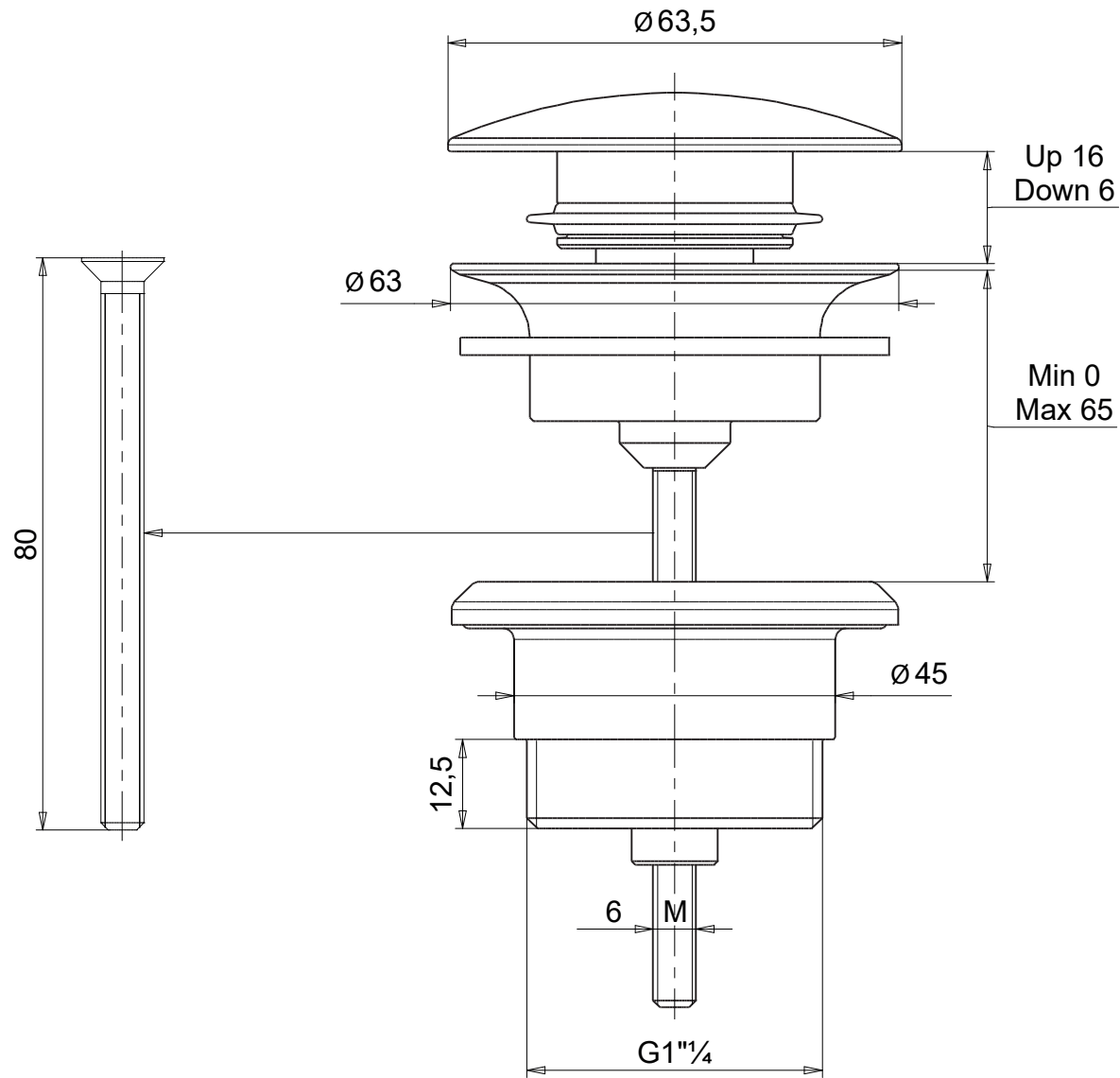
Universal Click Clack Waste
